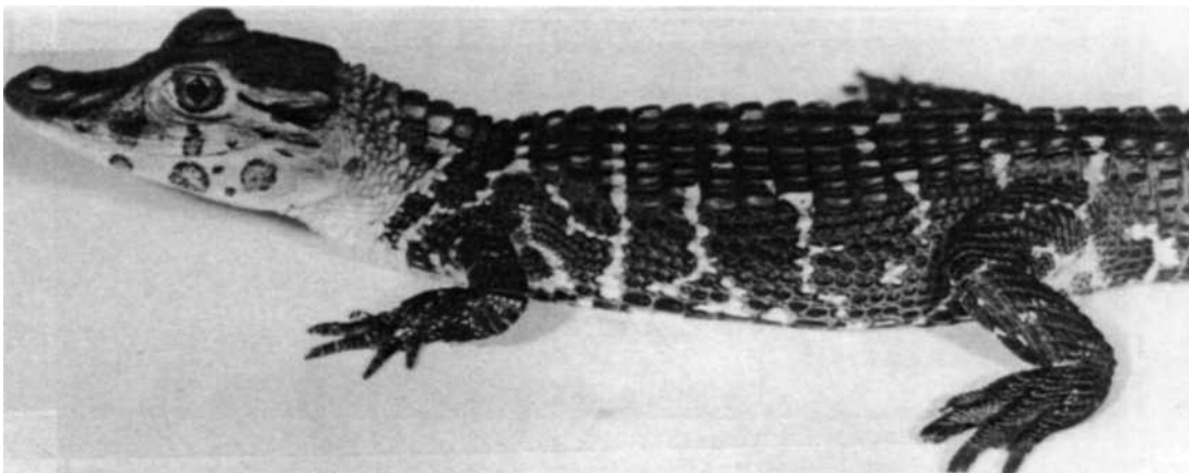
Figure 10. A and B. Flank sculation typical for Caiman latimstris : A. Illustrated. B. In life. C and D. Flank sculation typical for Melanosuchus niger , composed of at least five rows of alternating small and large round, poorly keeled scales. C. Note alternating rows of large and small scales illustrated. D. In life.
