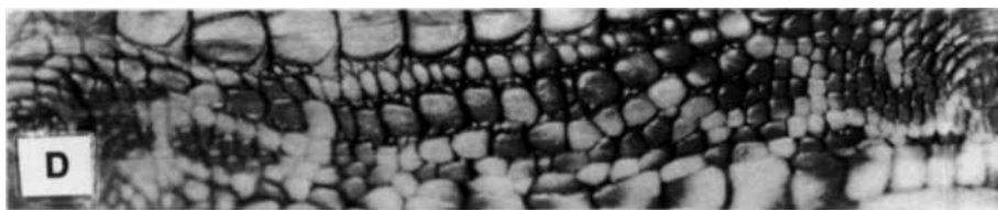
Figure 11. Flank scalation typical for C. crocodilus yacare . A. Diagrammatic. B. Raw dried skin. C. Tanned and finished skin. D. In life (juvenile).
