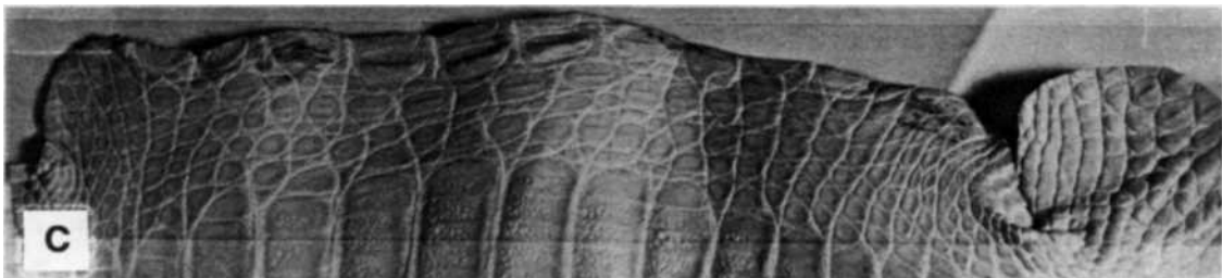
Figure 12. Flank sculation typical for C. crocodilus crocodilus . A. Diagrammatic. B. Raw dried skin. C. Crust tanned skin.
