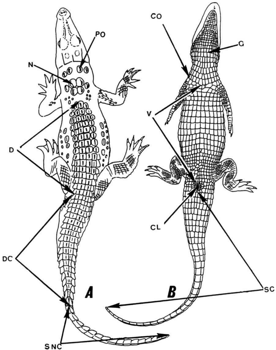
Figure 4. Body regions of crocodylians. A. SNC - single caudal verticils; DC - double caudal verticils; D - dorsal scales; N - nuchal scales; PO - post occipital scales. B. SC - sub-caudal scales; CL - anal opening or vent; V - ventral scales; CO - collar; G - gular region.
