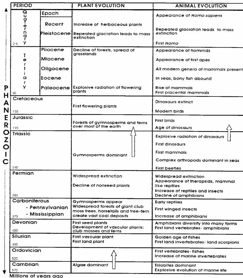
Figure 1 – Nature of life on Earth through time – from Wells (1996)
